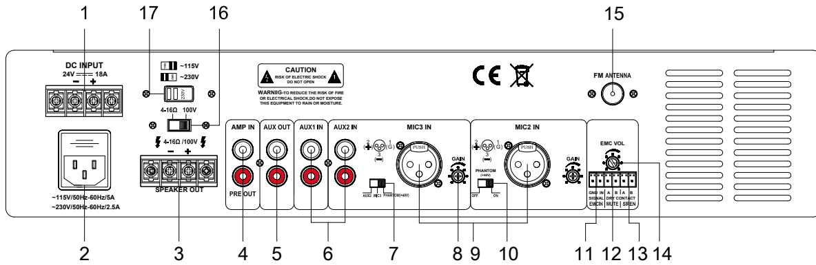
DMA350U/DMA500U/DMA650U Rear Panel
