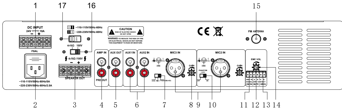
DMA350U/DMA500U/DMA650U Rear Panel
