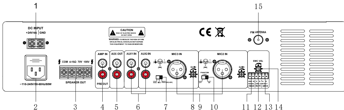
DMA60U/DMA120U/DMA250U Rear Panel
