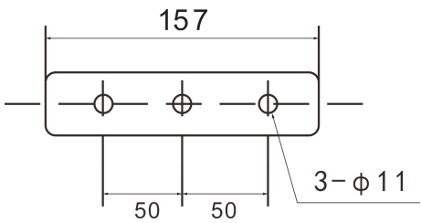
Mounting Bracket View
