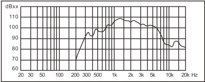
Frequency Response (dB SPL, 1W, 1m)
