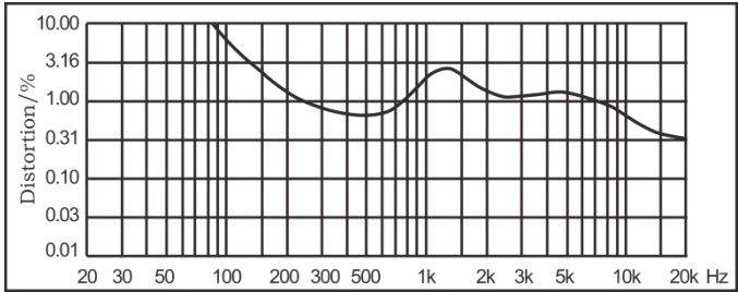
Distortion (THD<5% 1W, 1m, 200Hz-10kHz)
