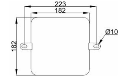
Base Plate Mounting Hole Diagram
