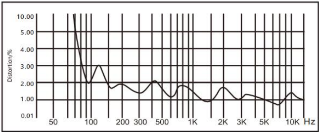
Distortion (THD< 5% 1W, 1m, 200Hz-10kHz)
