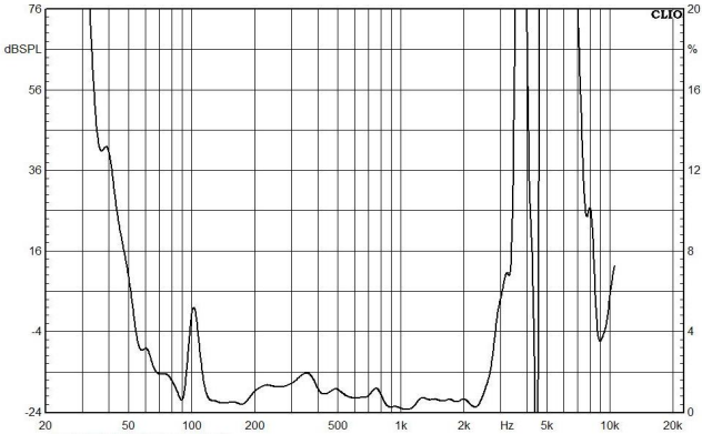
Distortion Curve:
