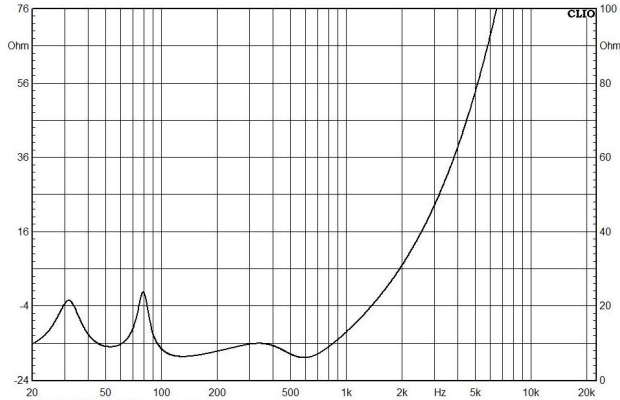
Impedance Curve:
